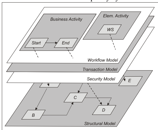
Figure 1 From Business service to structural model
