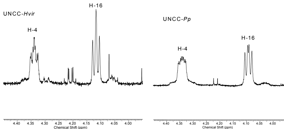
Figure 11. Proton spectra in the region of H-4 and H-16 of the UNCC – Hvir (left) and UNCC – Pp (right).
