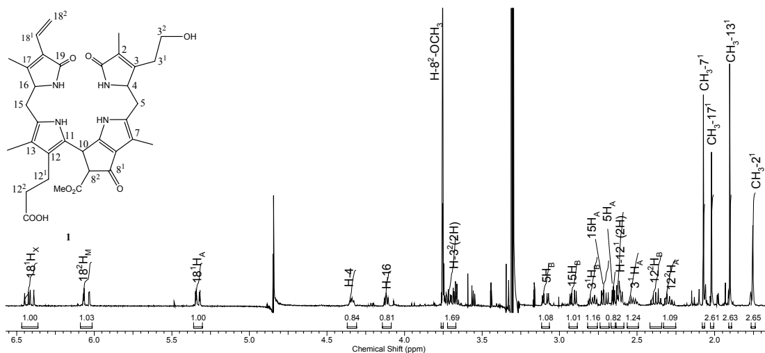
Figure 10. The high resolution proton spectrum of the UNCC – Hvir
